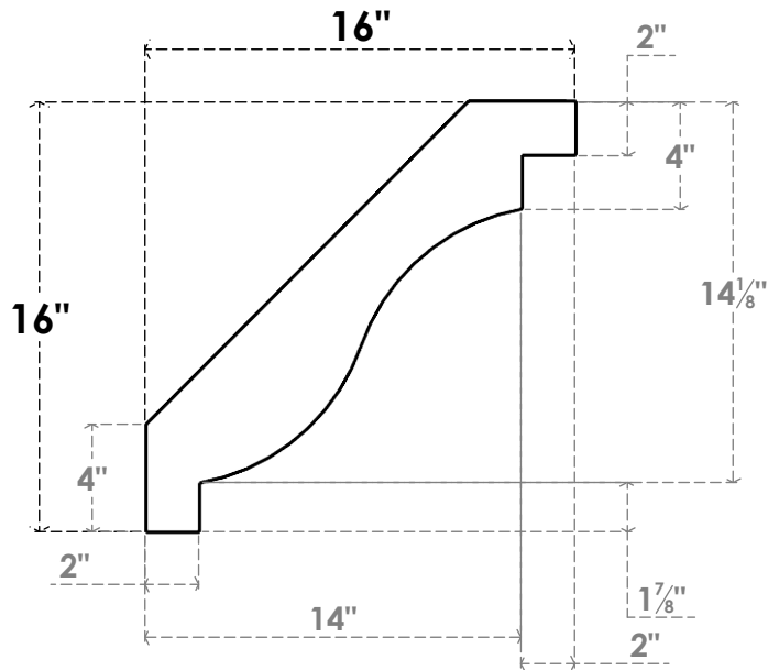
SIDE PROFILE
